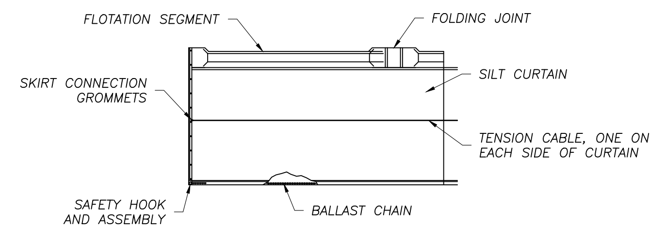
2 (TYP) FLOATING BOOM W/ OPTIONAL SILT CURTAIN NTS
